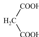
Malonic Acid
